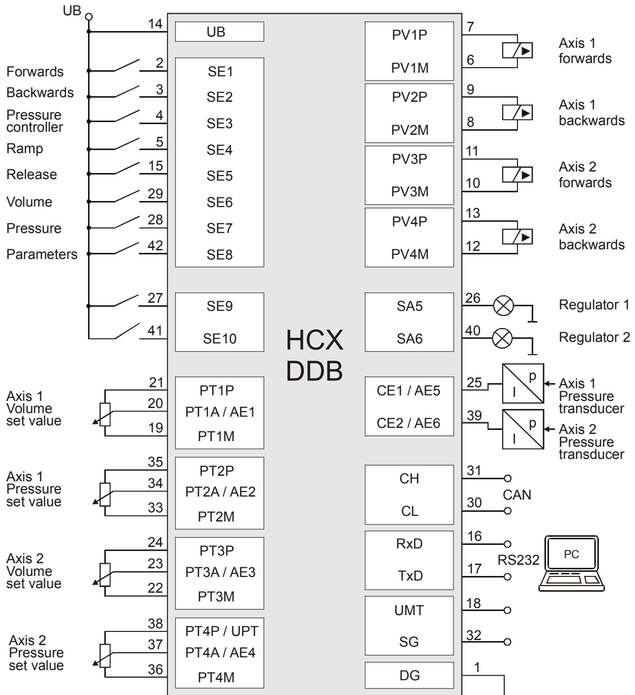
Connection Diagram
